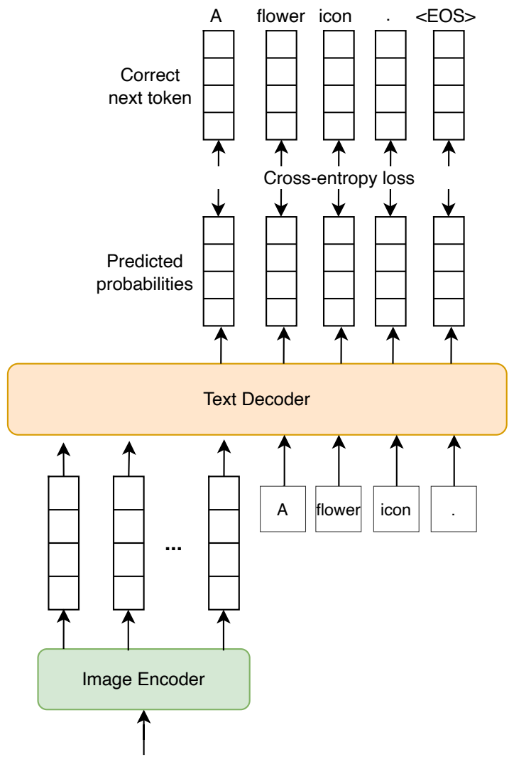
Figure 12: Loss calculation over the predicted probabilities
