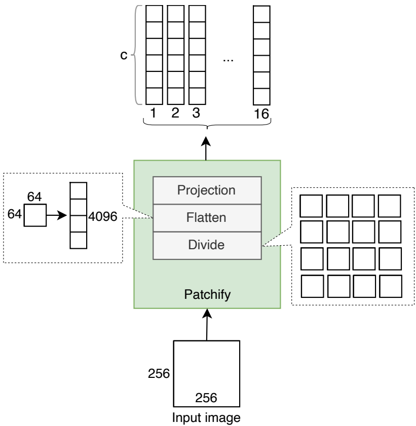
Figure 9: Patchification process
