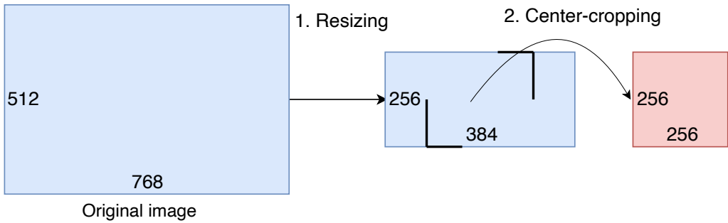
Figure 5: Resizing followed by center-cropping
