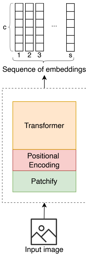
Figure 8: Transformer-based image encoding
