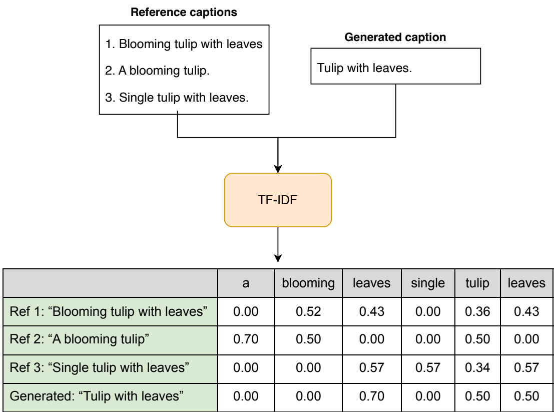
Figure 15: TF-IDF converting captions to numerical representations
