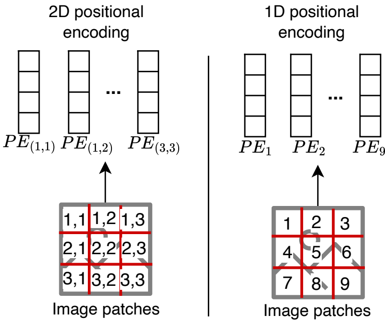
Figure 10: 1D vs. 2D positional encoding
