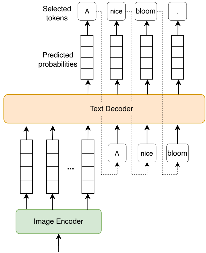
Figure 13: Generating a caption given an input image
