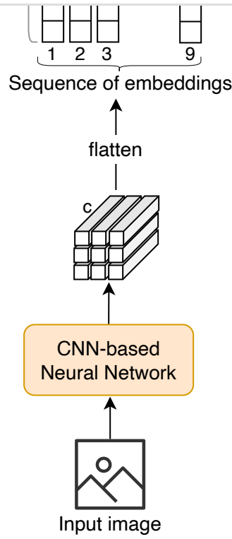
Figure 7: A CNN-based image encoding
