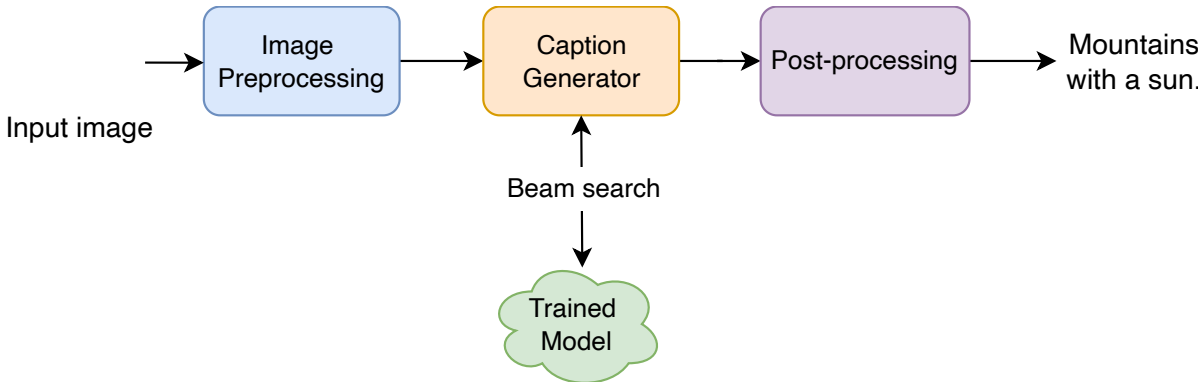
Figure 17: Image captioning overall design
